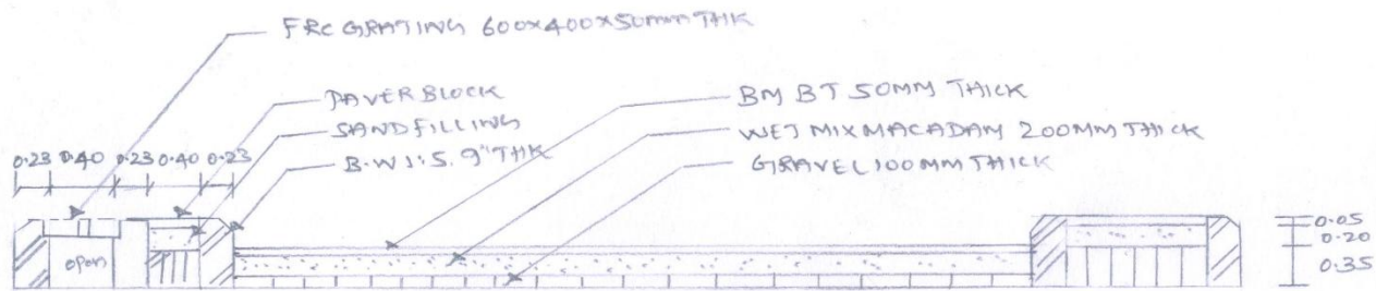
ROAD CROSS SECTION
